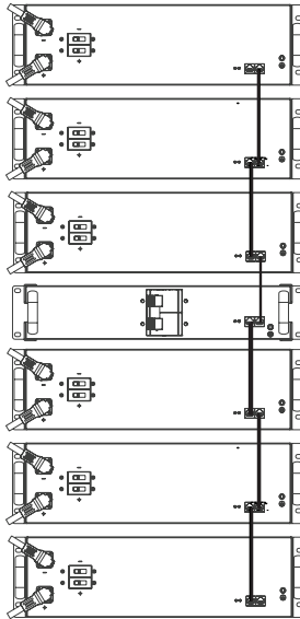
Figure 8. Six batteries with Battery Module Combiner
