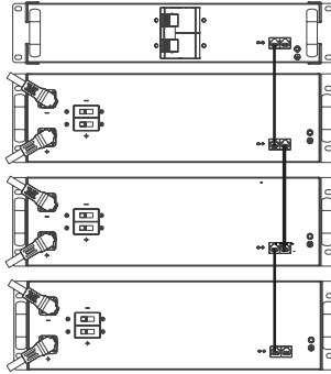
Figure 12. Grounding the Battery Module Combiner
