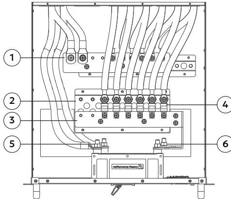
Figure 6. Battery Module Combiner with the top removed
